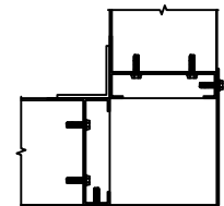
OPTION #1 BOXED CORNER
