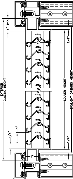
VERTICAL SECTION GLAZING FRAME OPTION
