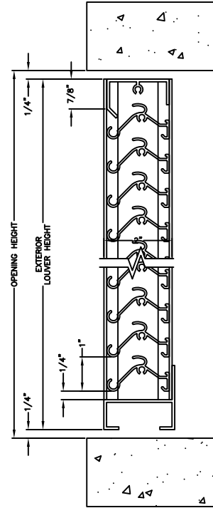
VERTICAL SECTION CHANNEL FRAME OPTION
