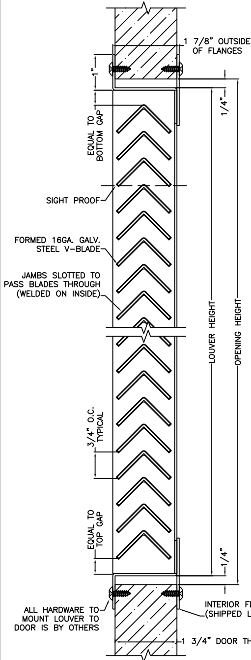
*SECTION VIEW*
