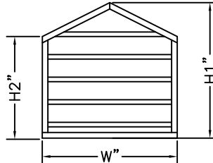
SHAPE D (DOUBLE SLOPED TOP)
