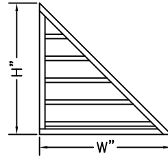
SHAPE B-R (RIGHT TRIANGLE - SLOPE RIGHT)
